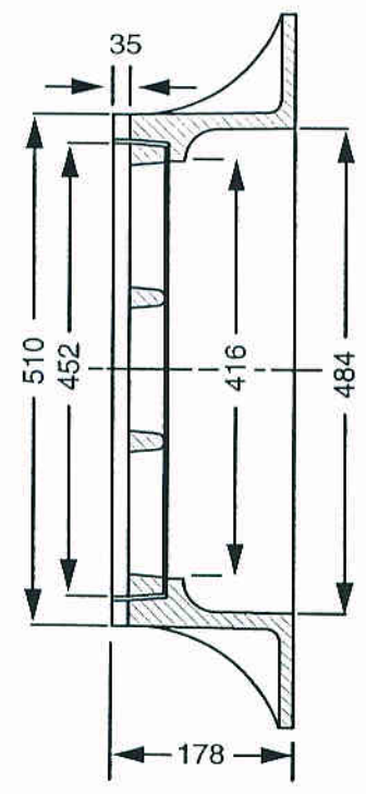
SECTION B-B
