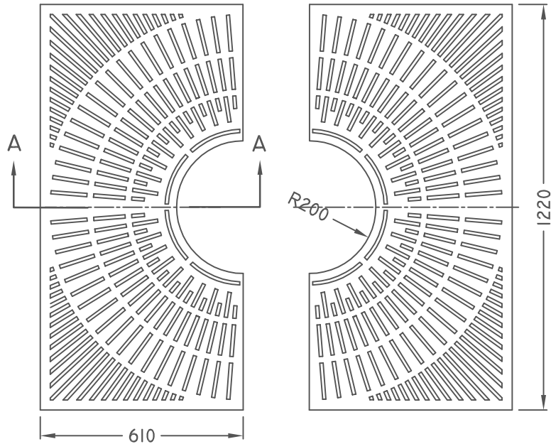
PLAN
